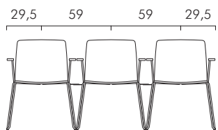
Cantilever frame. With armrests. Max 10 chairs.
