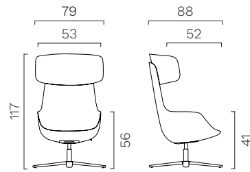
LARGE lounge armchair. Harmonic tilting lockable device.
