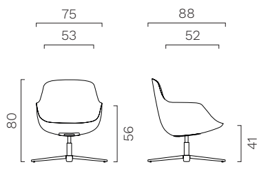
SMALL lounge armchair. Harmonic tilting device.
