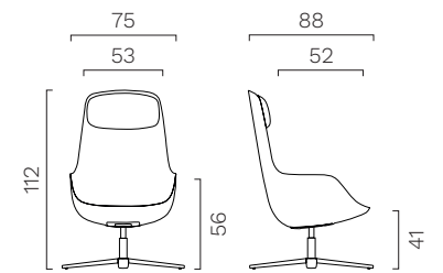
MEDIUM lounge armchair. Harmonic tilting device with automatic return.
