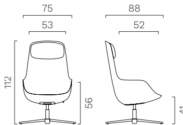
SMALL lounge armchair. Harmonic tilting lockable device.
