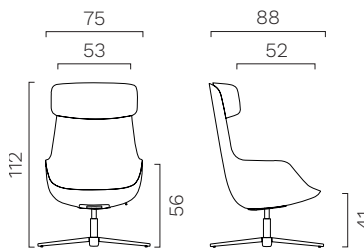
MEDIUM lounge armchair. Harmonic tilting lockable device.
