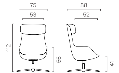
LARGE lounge armchair. Harmonic tilting device with automatic return.
