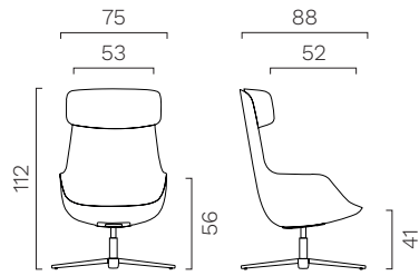
MEDIUM lounge armchair. Harmonic tilting device.
