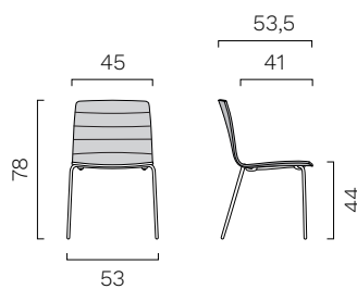
Polypropylene unibody with removable cover, without armrests. 4-leg frame.
