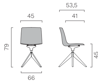
Upholstered polypropylene unibody. Wooden pyramidal base.
