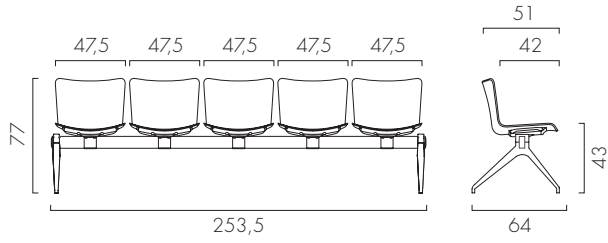
Banc 5 places
