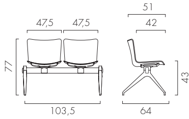
Banc 3 places
