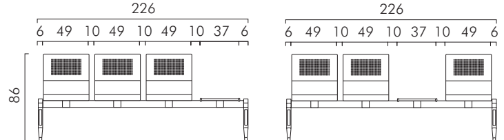
3-seater bench+table
