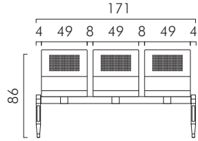
3-seater bench
