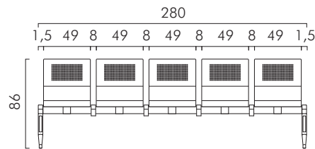
5-seater bench
