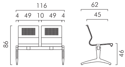
2-seater bench
