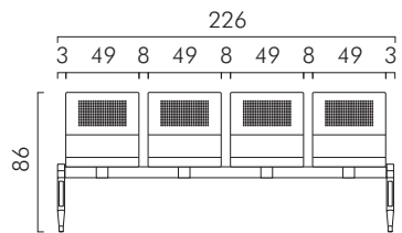
4-seater bench
